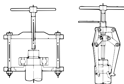
Fig. 15.12 Puller dismounting
