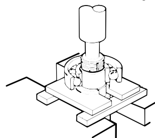
Fig. 15.13 Press dismounting
