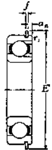
With Snap Ring NR
