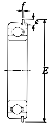
With Snap Ring 62NR
