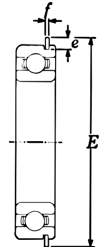
With Snap Ring 63NR
