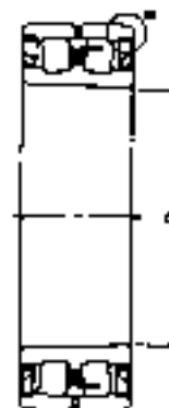
Tapered Bore MX-W222K Taper 1:12
